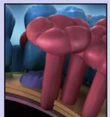
Neuraminidase
